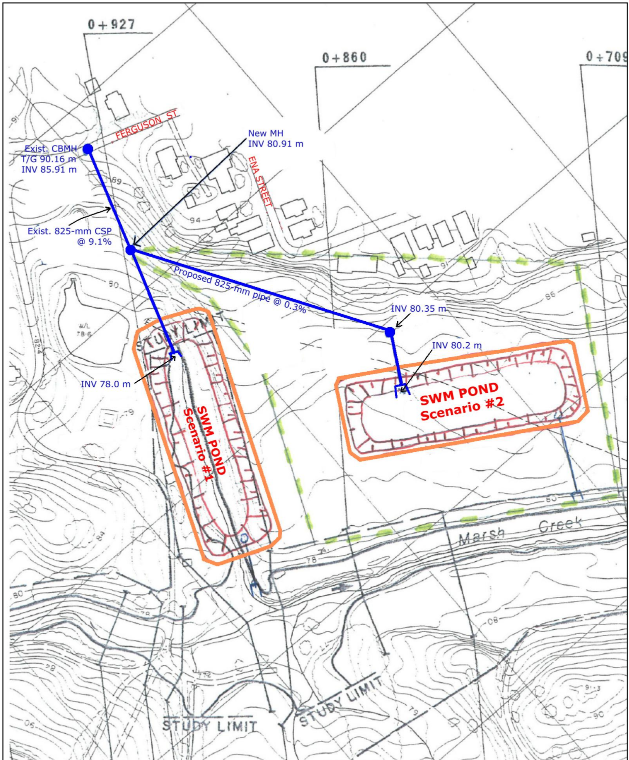
Appendix F: FIGURE F-2: P1 SWM Pond Facility Scenarios
